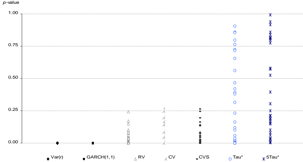
Figure 4: p -values for the 30 DJIA stocks, Jan. 1998 - Dec. 2002, 5-minute sampling
