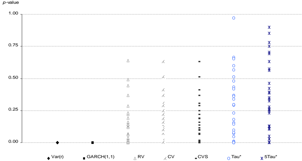
Figure 7: p -values for the 30 DJIA stocks, Feb. 2001 - Dec. 2004, 5-minute sampling
